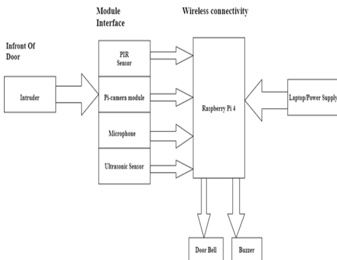
Fig-1: Architecture diagram of the proposed system
