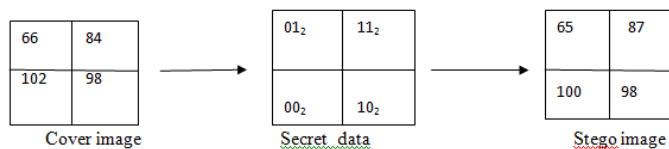
Figure: 2 LSB using 2 bit replacement method
