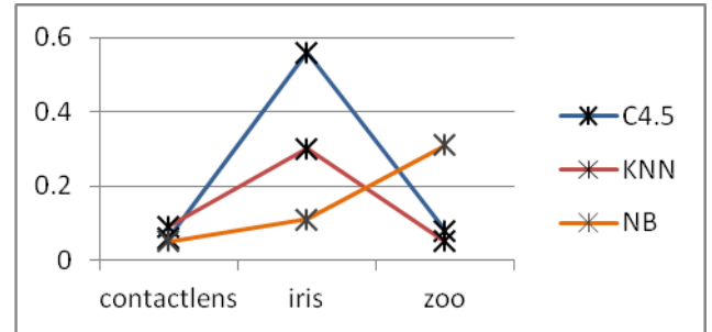
Figure 1. Wrapper selection time in sec between three datasets
