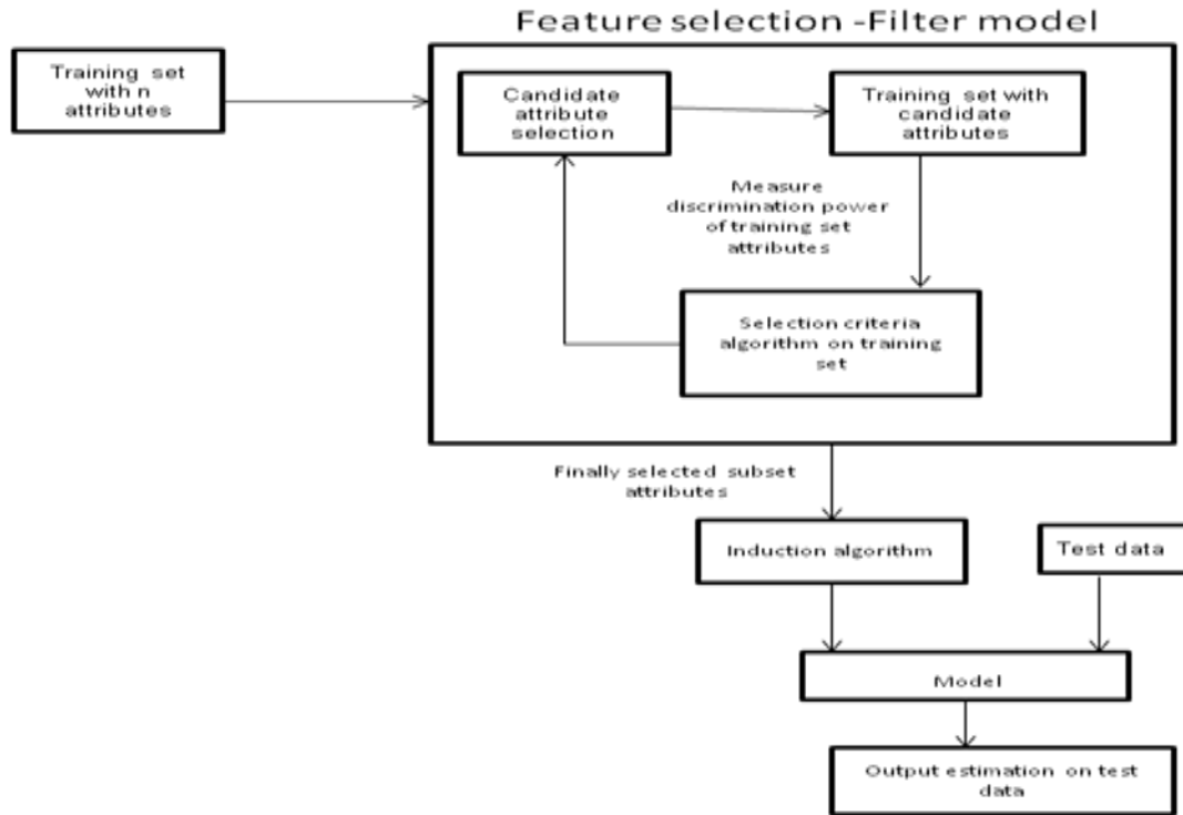
Figure: 1 Feature selection using filter model
