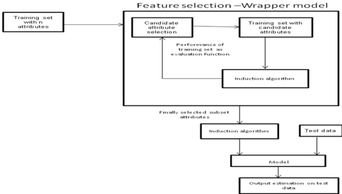
Figure 2: Wrapper model of feature selection Wrapper algorithm as given in [12]
