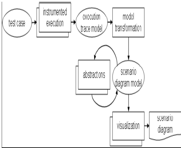
Figure 2. Reconstructing scenario diagrams.
