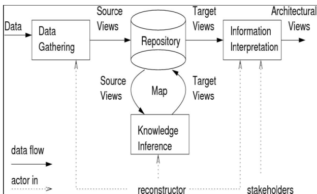
Figure 1. The reconstruction process.
