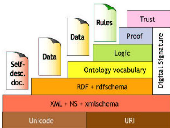
Figure 1: Semantic web mining architecture
