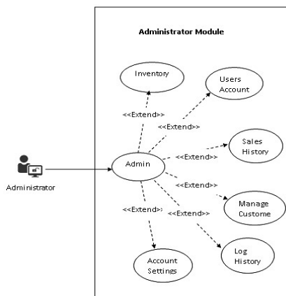
Figure.4 Use case diagram Administrator Module
