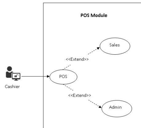
Figure.6 Use case diagram POS Module
