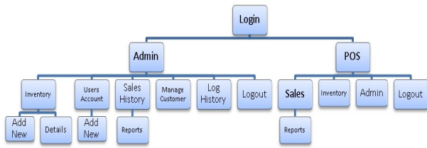
Figure.3 Hierarchical Input Process Output
