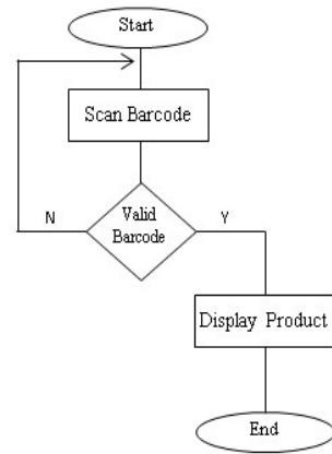
Figure.9 Barcode Scanner Flow Chart
