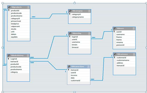
Figure 12 Database Schema
