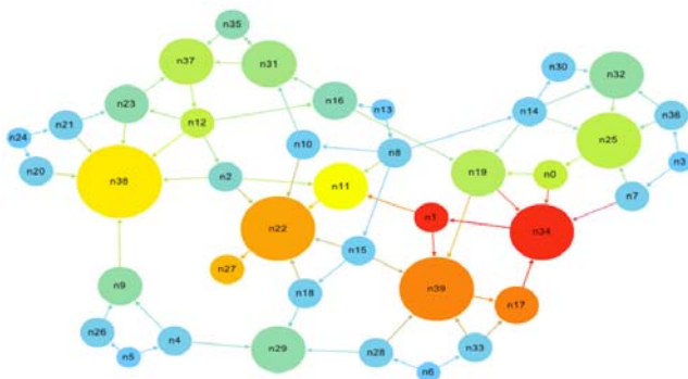
Figure 5. Page Ranking
