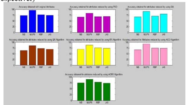
Figure 2: Comparison of Accuracy for different Classifiers by using attributes obtained by Existing and Proposed Algorithm
