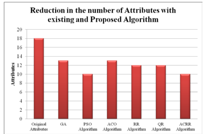
Figure 1: Reduction in the number of Attributes.
