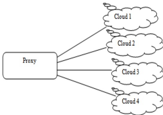
Figure 4. Normal operation
