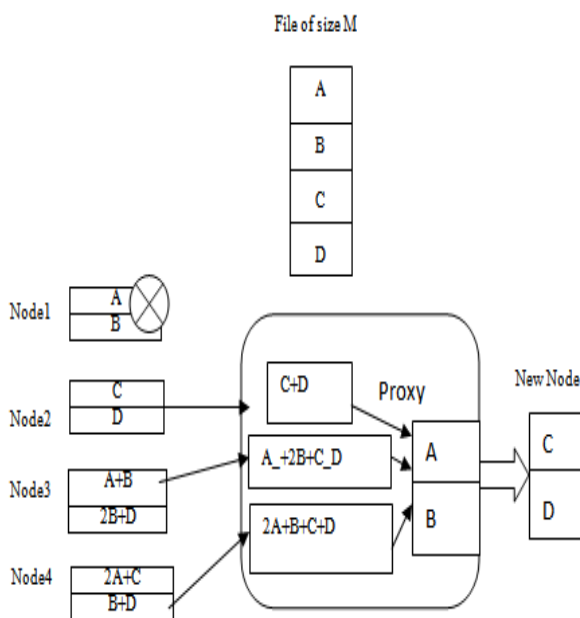
Figure 2. EMSR
