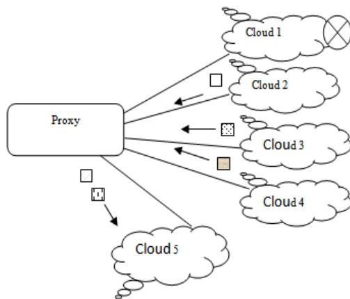
Figure 5. REPAIR OPERATION
