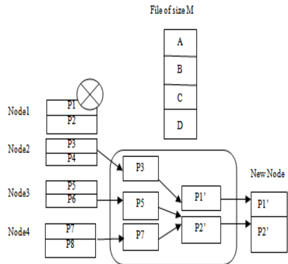
Figure 3. FMSR
