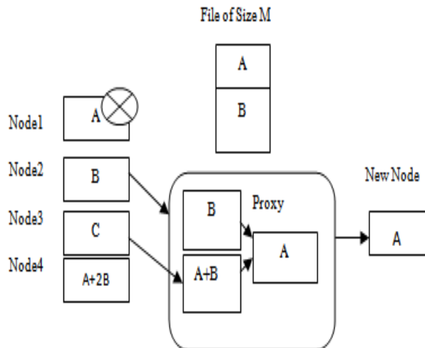
Figure 1. RAID-6
