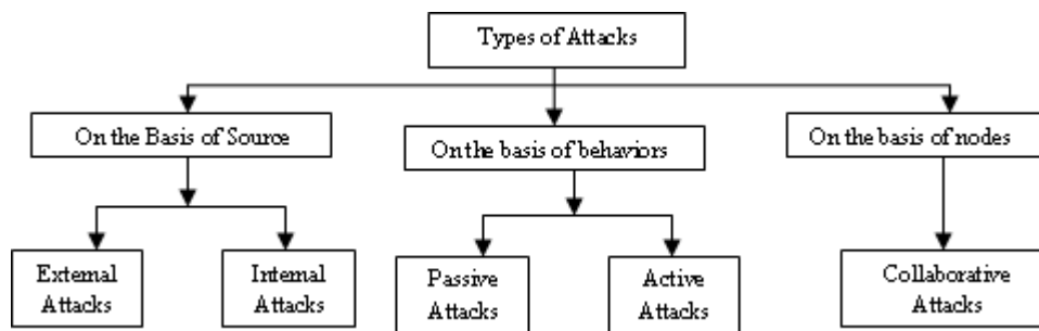
Figure 3: Categorization of Attacks in MANETs
