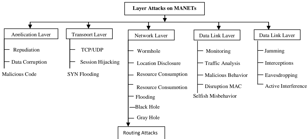
Figure. 2: Attacks in various layers of MANET
