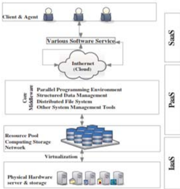
Figure 1: Cloud Computing Framework
