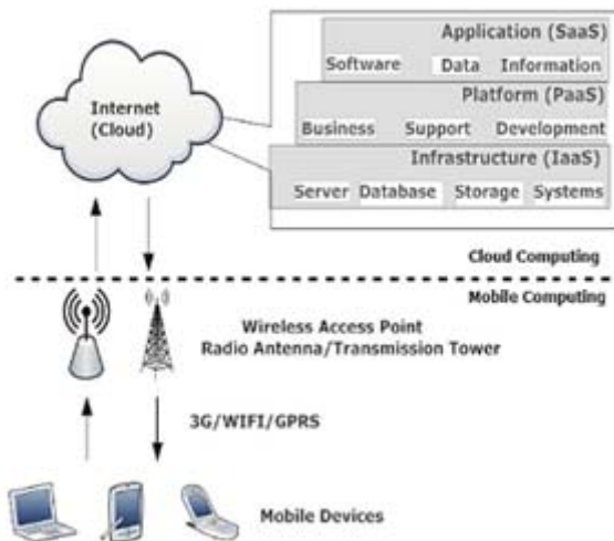
Figure 2. Mobile Cloud Computing (MCC) Architecture.
