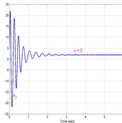
Figure 3. Constant Tracking Problem for x_2
