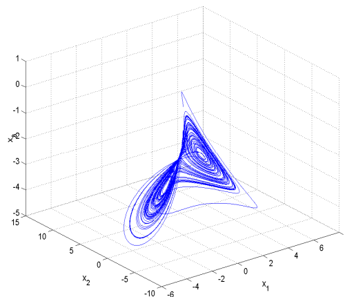
Figure 1. State Orbits of the Liu-Chen-Liu System
