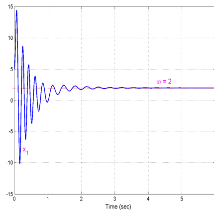
Figure 2. Constant Tracking Problem for x_1
