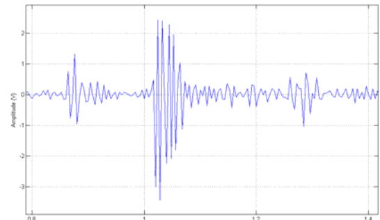
Figure 7 Cropped signal
