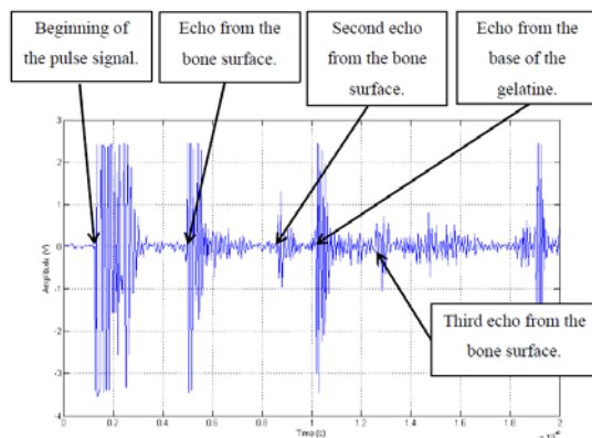
Figure 6 Echo signal identification
