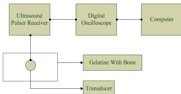
Fig.3 Top view Block diagram of experiment setup
