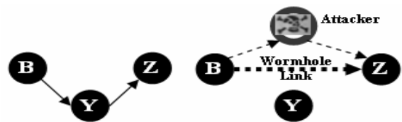
Figure 3: Wormhole Attack
