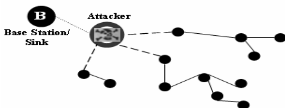
Figure 1: Sinkhole Attack
