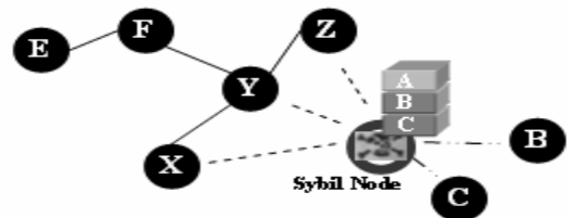
Figure 2: Sybil Attack
